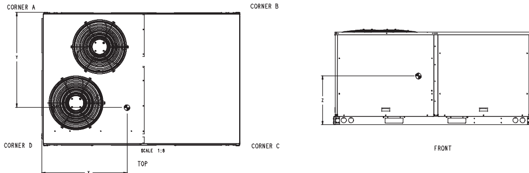
Dimensions 50TCMD08/09
